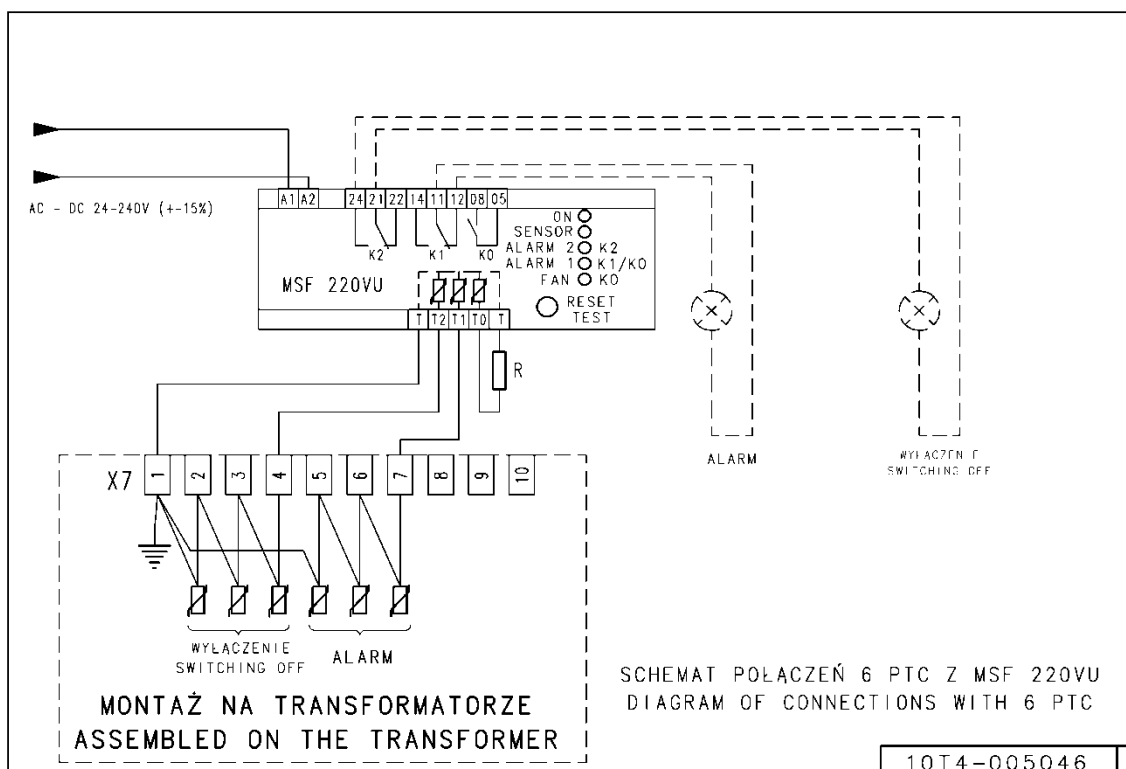
Fig. 13. Application diagram for temperature relay MSF 220VU.
