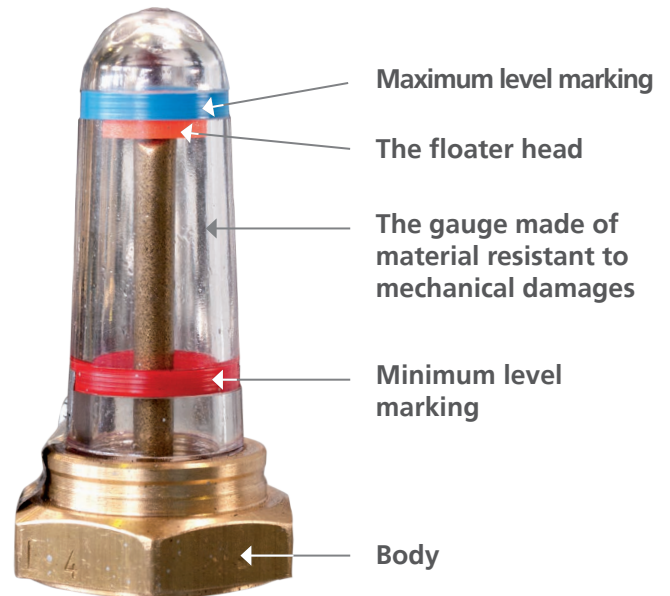
Fig. 10. Oil level indicator
