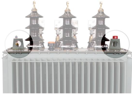
Fig. 3. Lifting lugs
